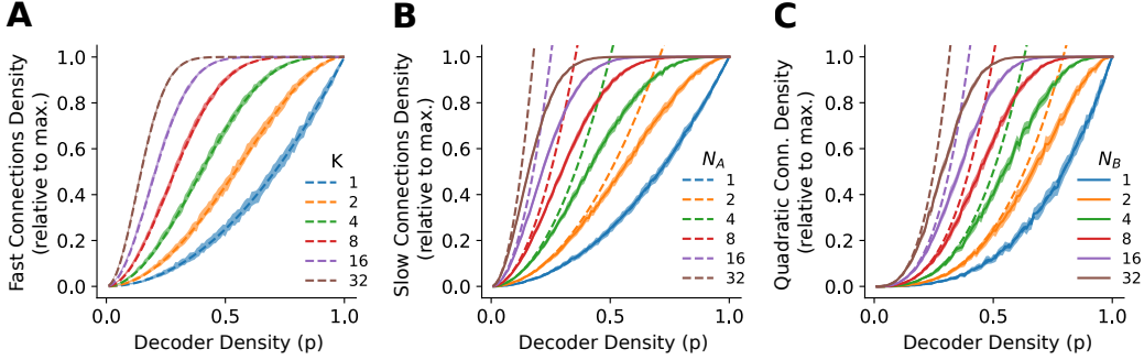
Figure 4: Expected number-connectivity density relative to all-to-all connectivity for the different synapse types as a function of connections the decoder density p . Solid lines illustrate mean across iterations, whereas shaded areas represent \pm 1 standard deviation from the average of the simulated connectivity (see Methods 7.8). Dashed lines correspond to theoretical upper bounds (Eq. 8-10). (A) The connectivity density for the fast synapses for different signal dimensions ( K ), (B) The connectivity density for the slow synapses due to linear computation (i.e. \sim N_A p^2 ), and slow multiplicative for different linear dynamical system densities (quadratic N_A synapses), (C) as a function of the decoder density p for different signal dimensions slow multiplicative ( K quadratic) and synapses for different quadratic dynamical system density densities ( N_B ). N_A for the linear part and N_B for represent the quadratic part, each representing the number of non-zero entries of matrices A and B respectively. Dashed lines represent the theoretical upper bounds, whereas shaded areas represent \pm 1 standard deviation from the average of the simulated connectivity (see Methods 7.8).
