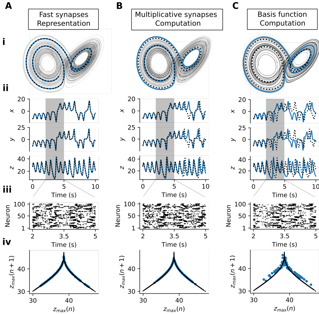
Figure 2: Implementation of a Lorenz dynamical system. Across columns: (A) The numerical solution was found using an explicit Runge-Kutta method of order 4. The network contains only fast synapses and receives as input the output of the Lorenz simulation, which the network read-out tracks closely. (B) A network with multiplicative synapses (mSCN) computing the Lorenz attractor through its network dynamics. (C) A network with nonlinear basis functions computing the Lorenz attractor through its network dynamics. Across rows: (i) 3D view of the network readout for 100 sec (grey). The dotted line shows the 'true' simulation in the 2-5sec period, and the blue line shows the corresponding network output trajectory. (ii) Each network readout dimension (blue) across time vs the 'true' solution (black dotted). The gray region indicates the 2-5sec period used in panels i and iii. (iii) Raster plot with spikes emitted by the neurons in the time interval 2 - 5 sec. (iv) Peak analysis over 100 sec: blue = network output, black = 'true' Lorenz simulation.
