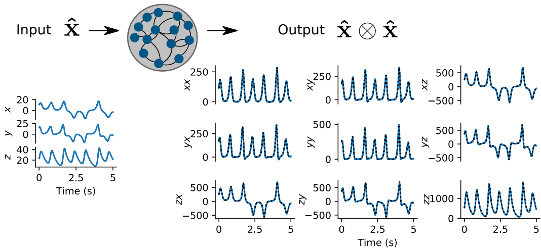
Supp. Fig. 2: Representation of the Kronecker product of the input. The Input \hat{\mathbf{x}} was given by a network which computed a Lorenz system. The second network, using eq. (23), outputs a signal \approx \hat{\mathbf{x}} \otimes \hat{\mathbf{x}} . Blue lines represent network output, black dotted lines represent the real \hat{\mathbf{x}} \otimes \hat{\mathbf{x}} .
